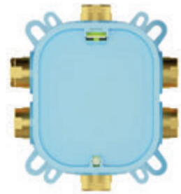
Two integrated water levels for easier installation
